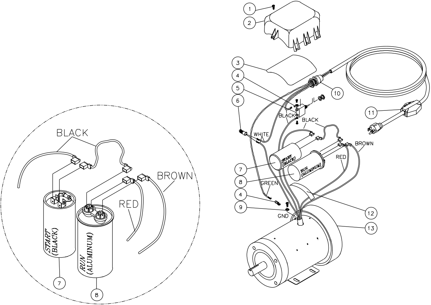
CAPACITOR TERMINAL ASSEMBLY
